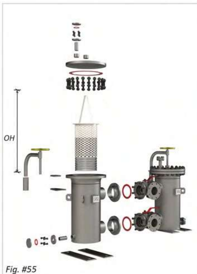
Duplex Strainers with 3-way Ball Valves - RF - #150
