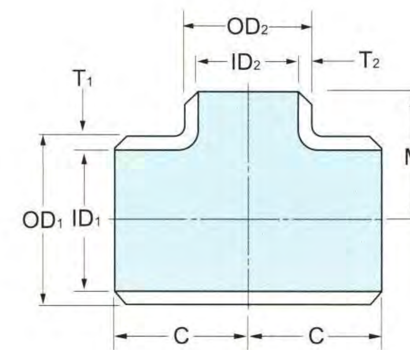
Reducing ( I )
