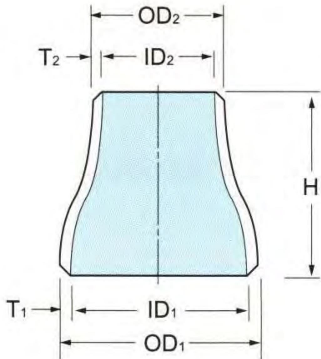
Concentric
