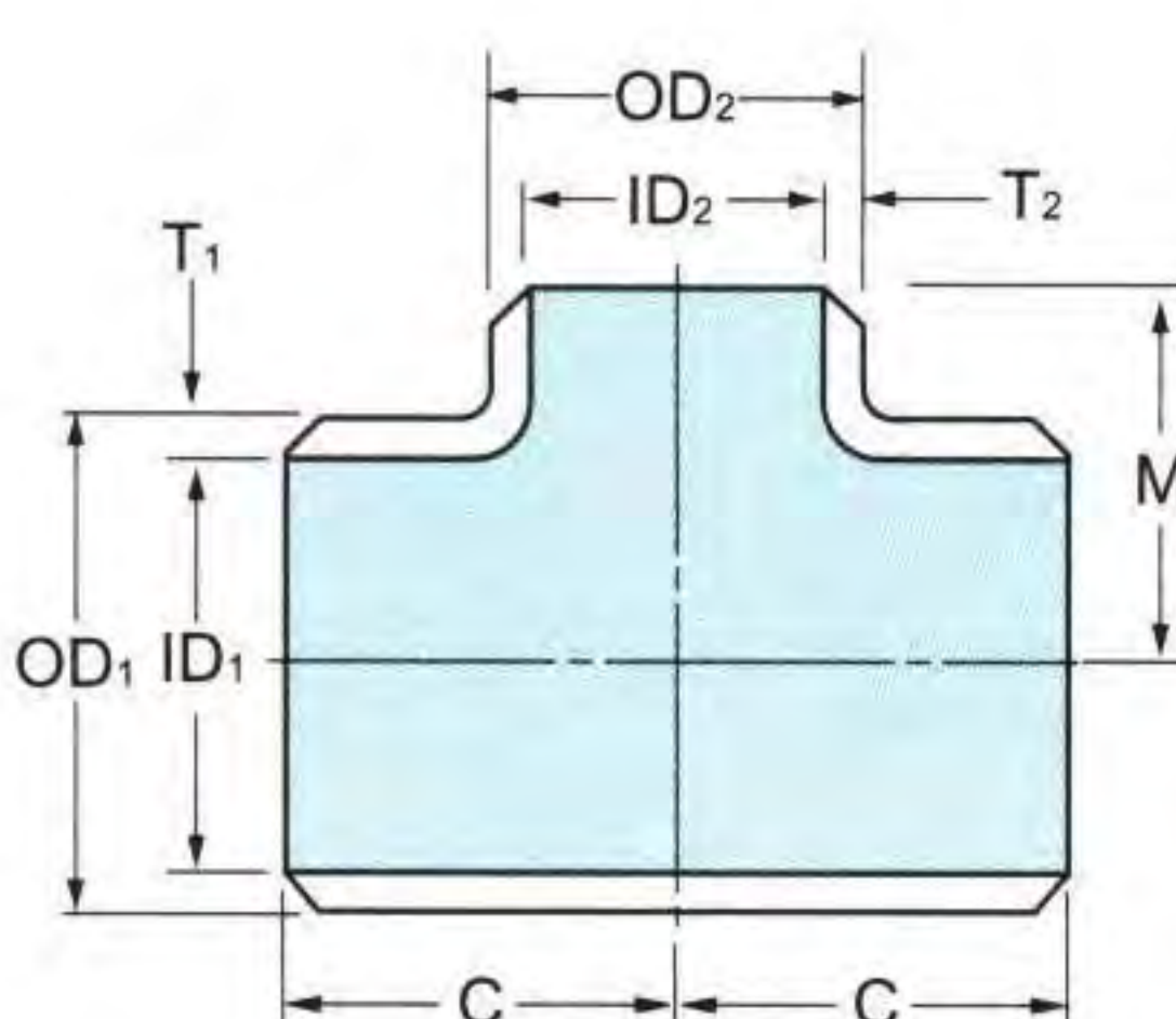
Reducing ( I )
