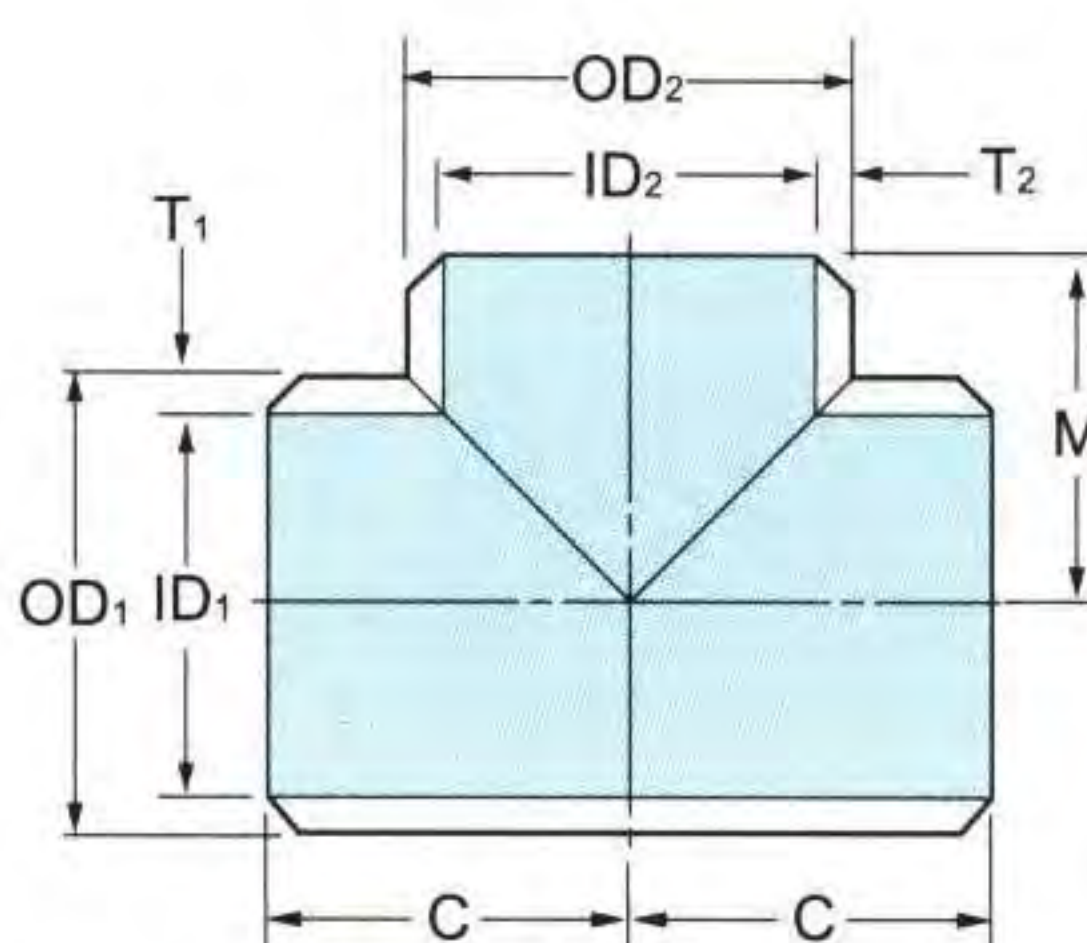
Straight ( II )
