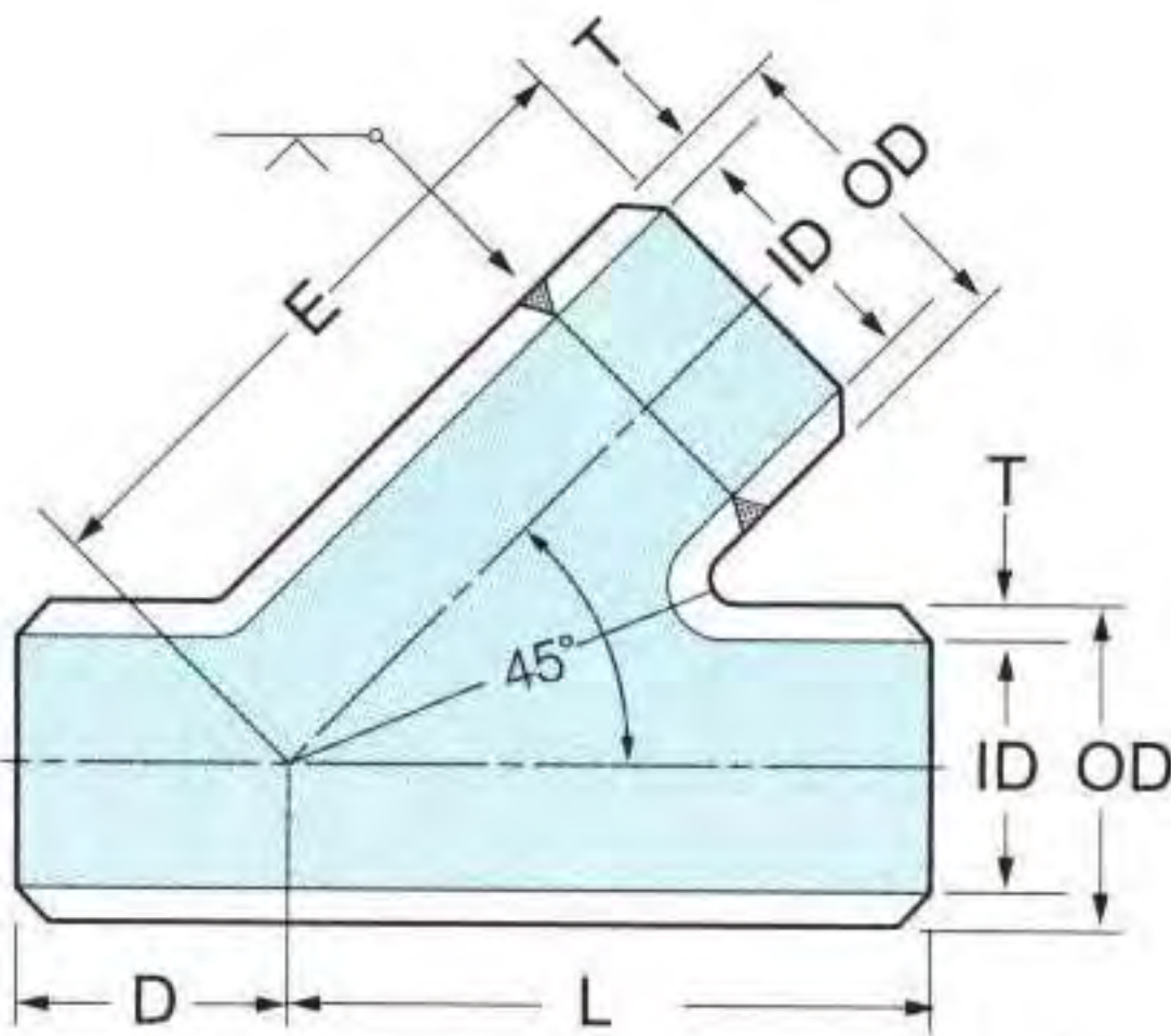
Type A
