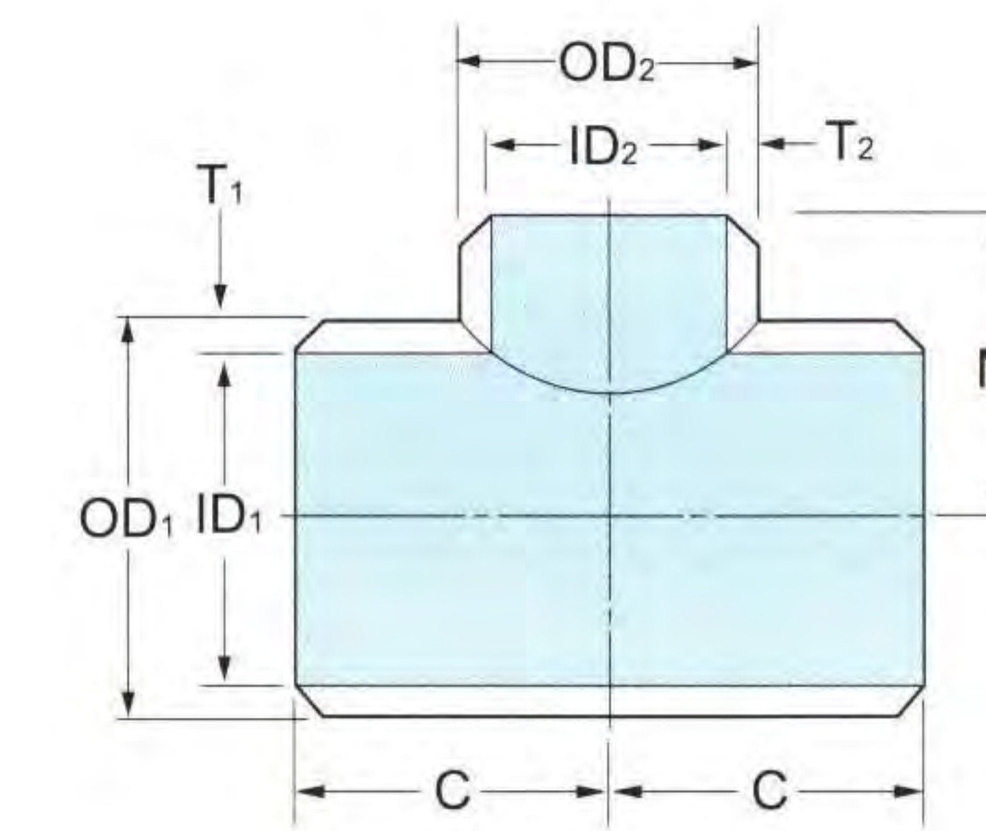
Reducing ( II )
