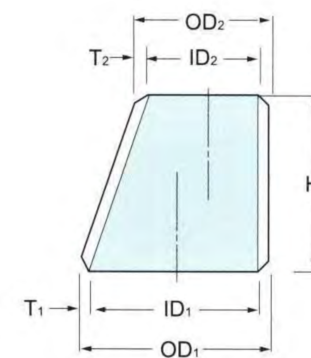
Eccentric
