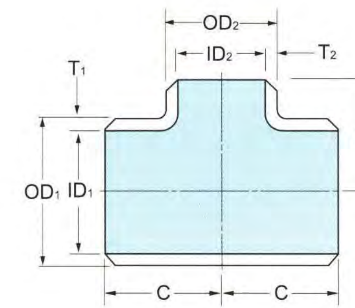
Reducing ( I )
