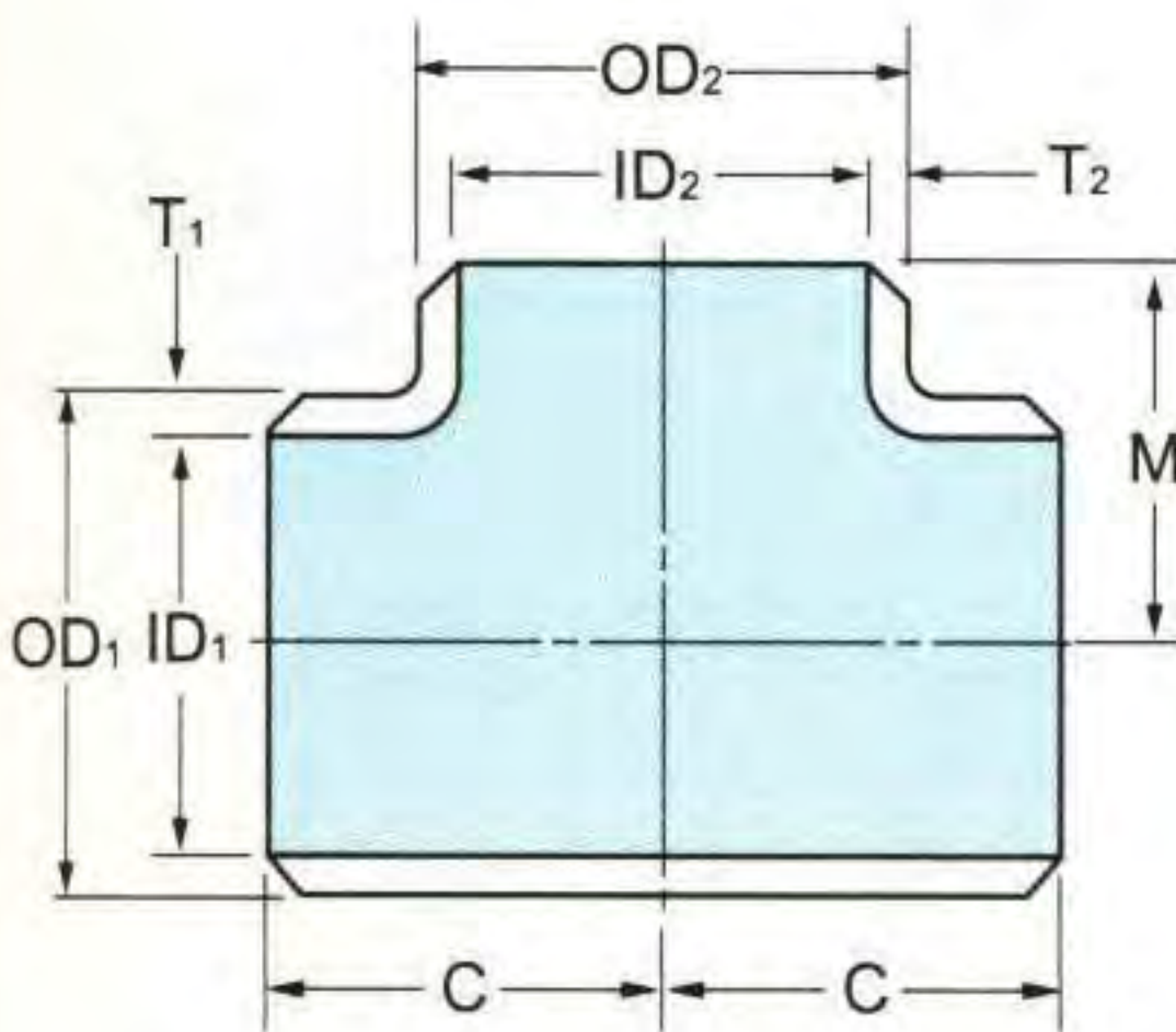
Straight ( I )
