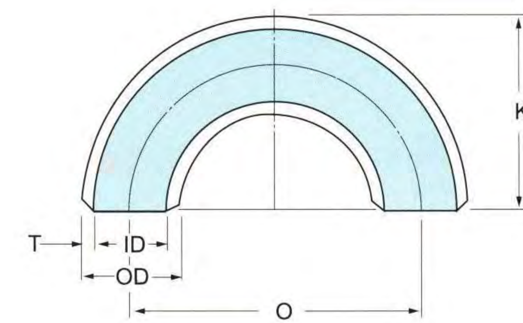
180° Elbow
