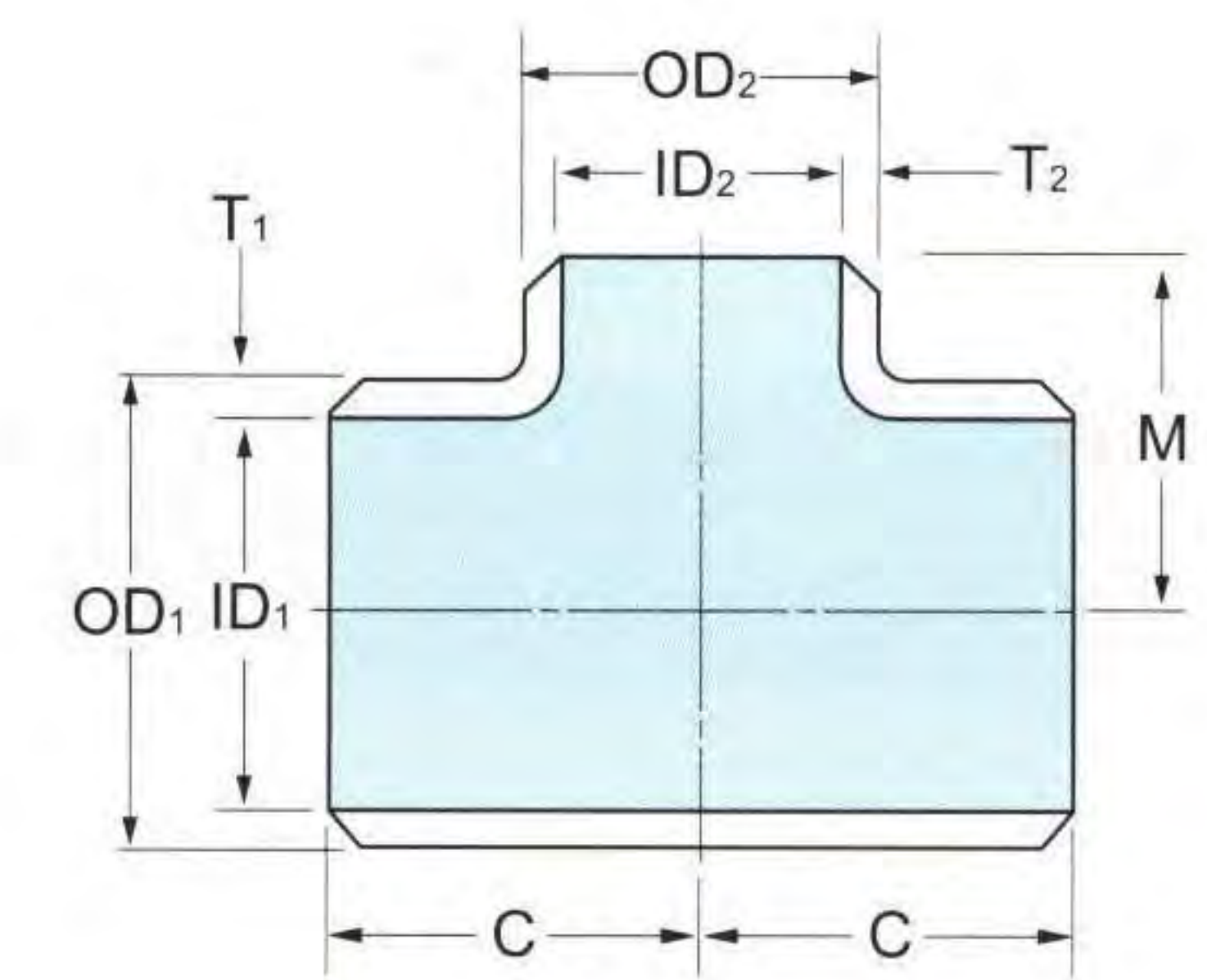
Reducing
