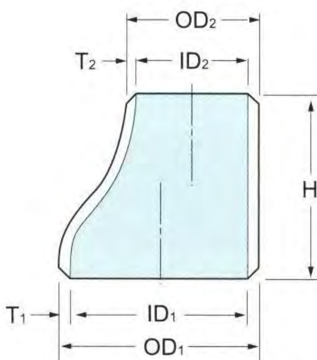
Eccentric
