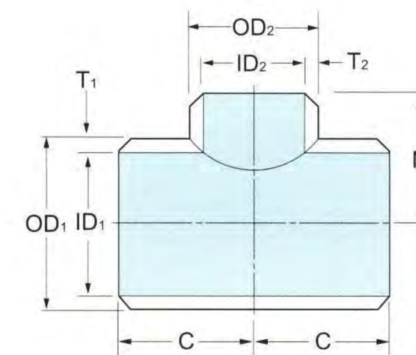
Reducing ( II )
