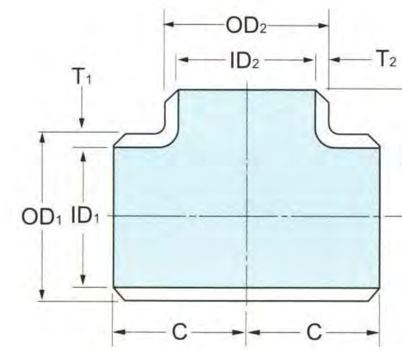
Straight
