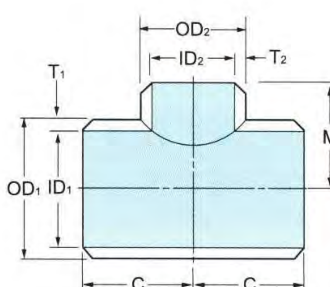
Reducing ( II )
